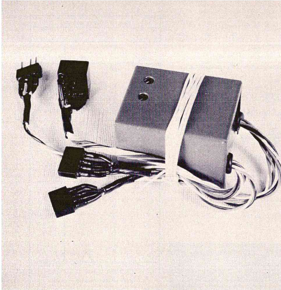
The completed receiver-decoder with all plugs attached. One of the smallest units available today.
