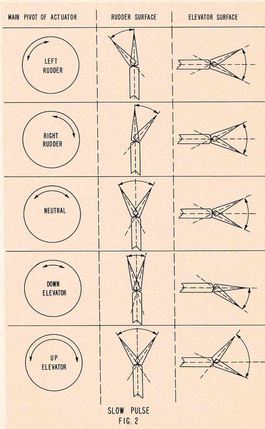
Adjustment of actuator and actual control surface for galloping ghost system, average position of control surface is the effective control position.
