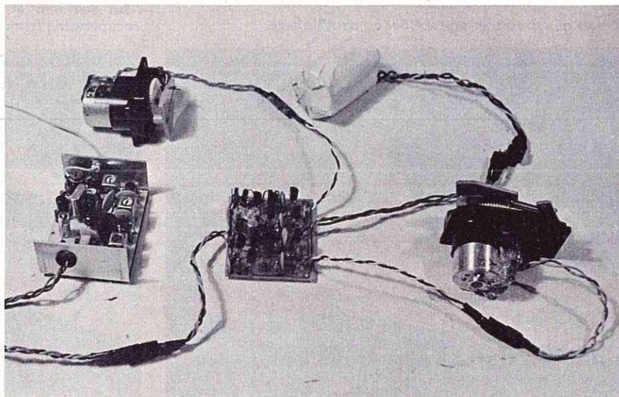
FIGURE 9: The complete system with two Rand actuators, Controlaire receiver, decoder, and light-weight battery pack.
