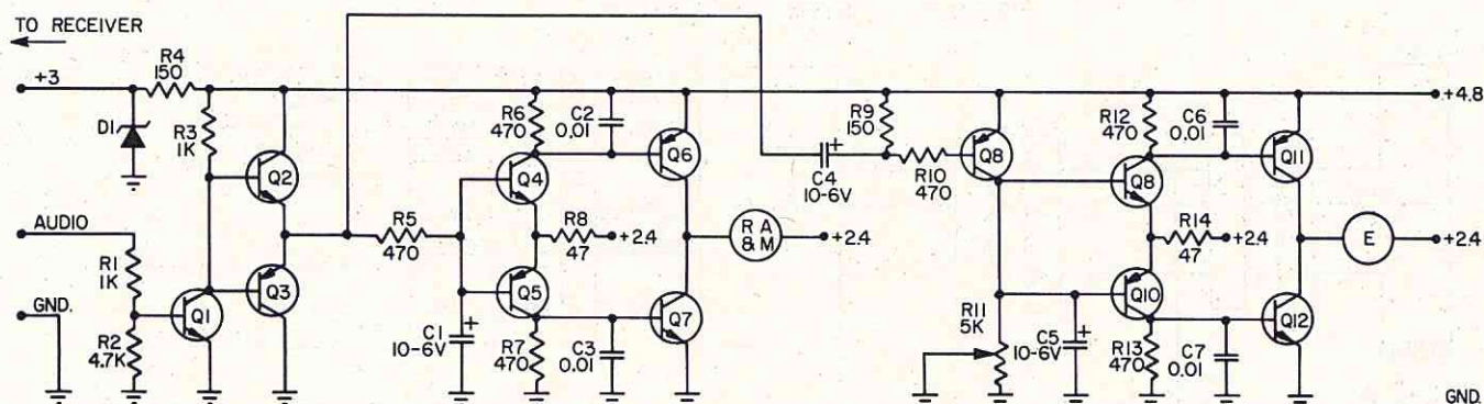
FIGURE 4. COMPLETE SCHEMATIC
