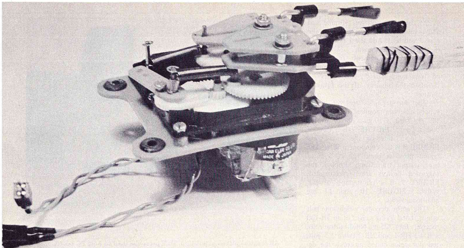
A close-up photo of a method for easily obtaining coupled ailerons and rudder using a Rand actuator. Two Rand rudder plates are stacked and spaced 3/16" using the ferrules supplied in a Rand mounting kit and are held together with 3-48 x 1/2" machine screws using lock washers. Kwik-Links connect to the ailerons. This particular system used in the author's low-wing Rodent. The elevator pushrod is not connected in this photo.
