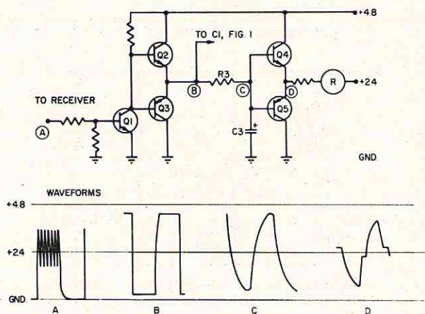
FIGURE 2. PULSE AMPLIFIER ADDITION
