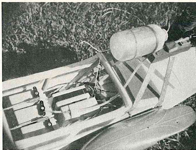
Seafoam equipment installation showing Kraft servos. Rand Swing'N Keepers used.
