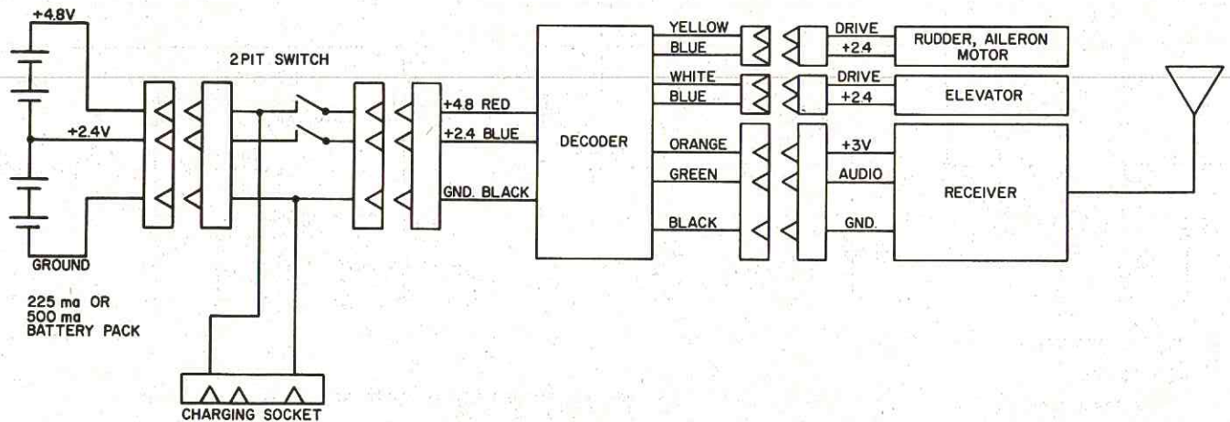
FIGURE 6. SYSTEM WIRING DIAGRAM
