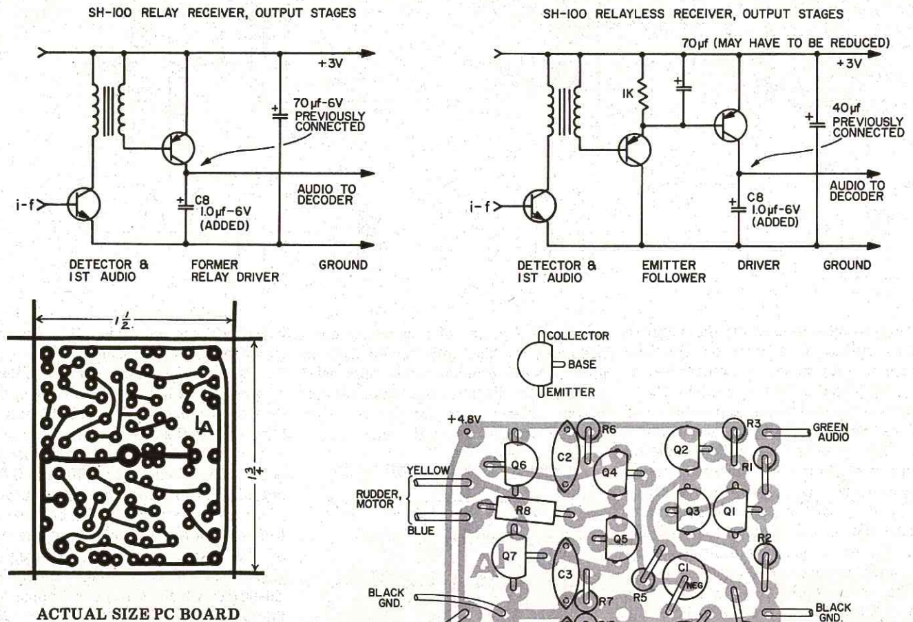
FIGURE 5. RECEIVER MODIFICATIONS
